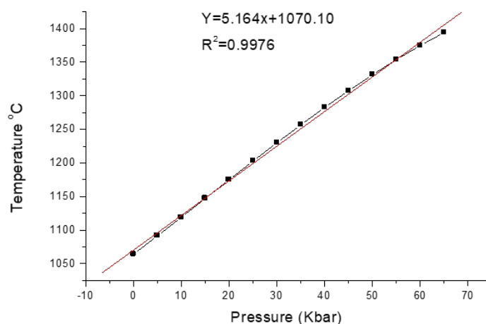
Figure 1: Melting Temperatures against Pressures for Gold from Itagunmodi.
